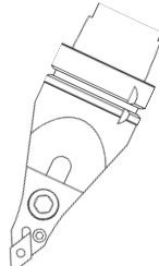
MCD' HSK-A63F.77 PDNNN 140.15
